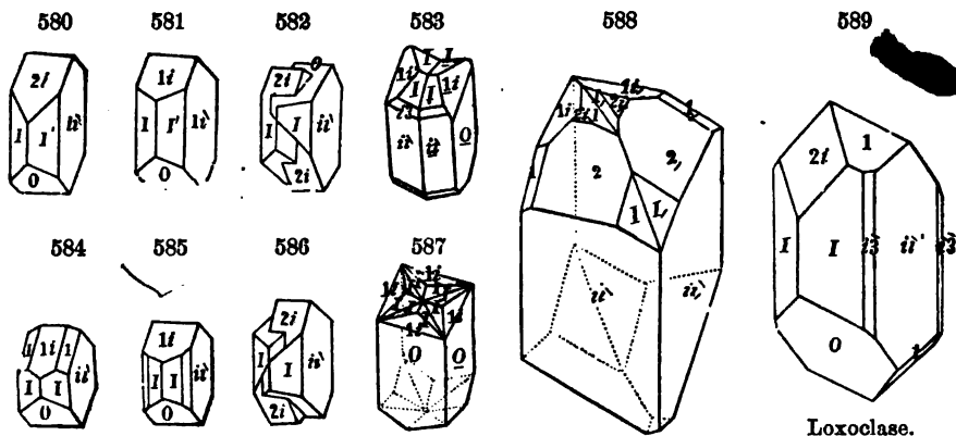
Loxoclase.
